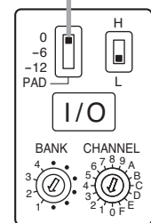
Pad switch
