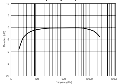
Frequency Response
