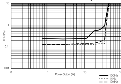
THD vs Power Output
