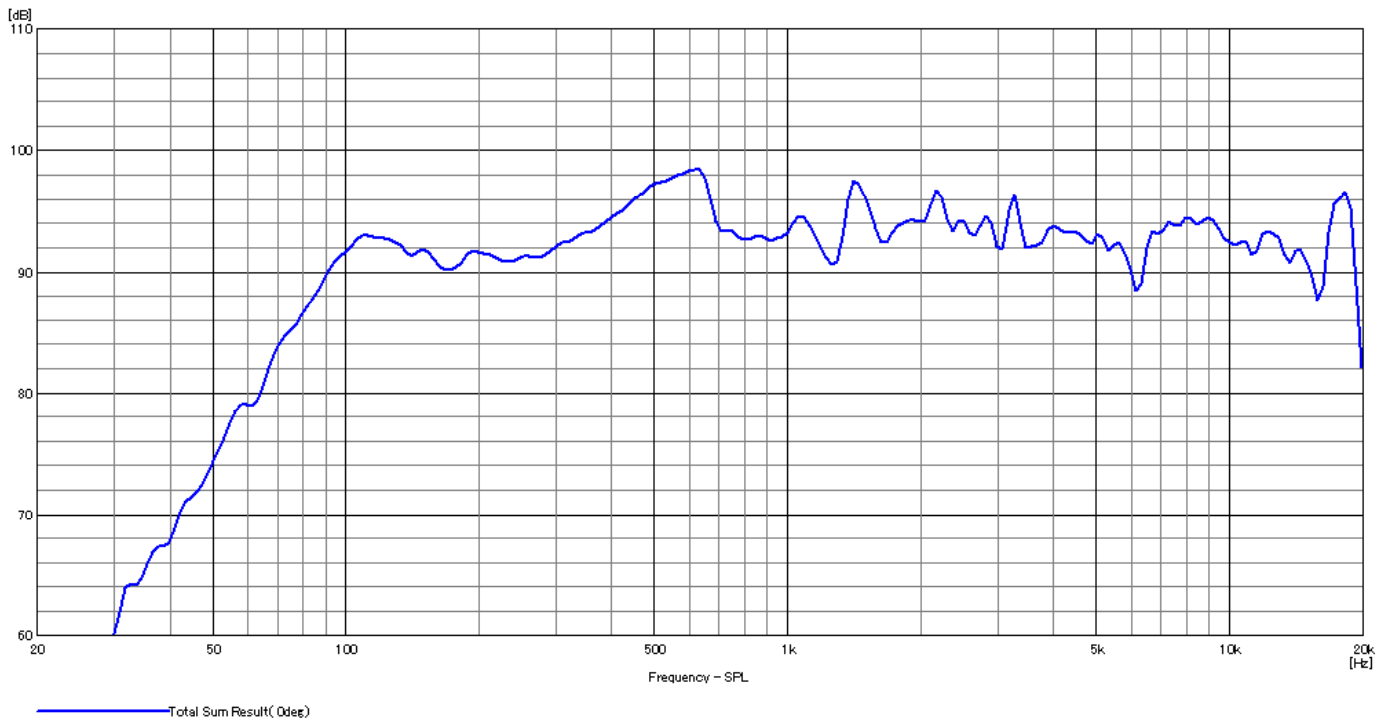
HS-1200 Frequency - Response
