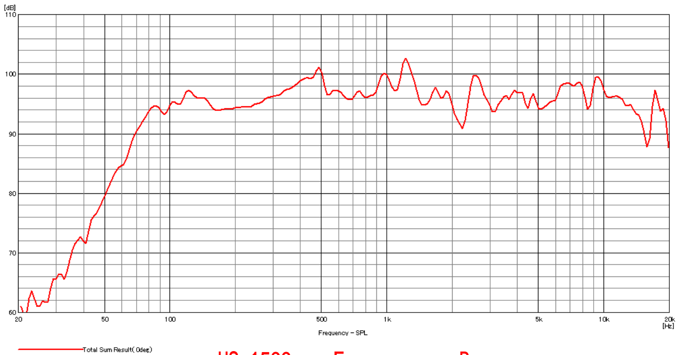
HS-1500 Frequency - Response
