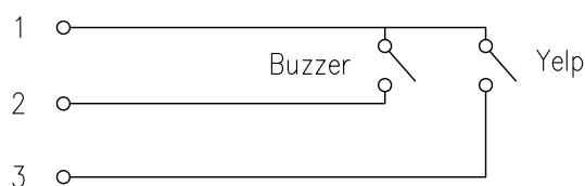
Connection Diagram
