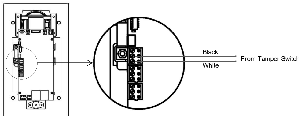
N-SP80AS1/VS1 (Rear)
