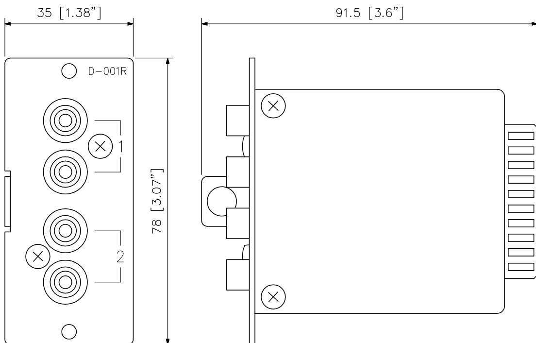
Front View
