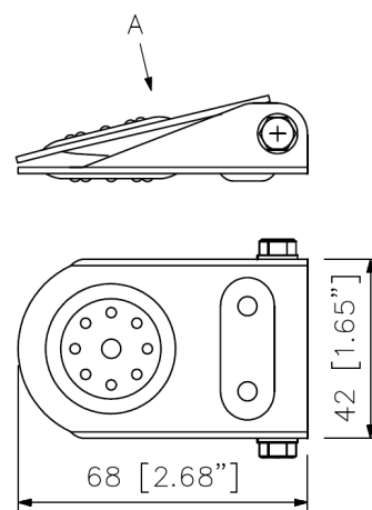
Satellite speaker mounting bracket
