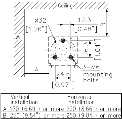
Dimensions of wall mounting hole (base bracket (accessory))
