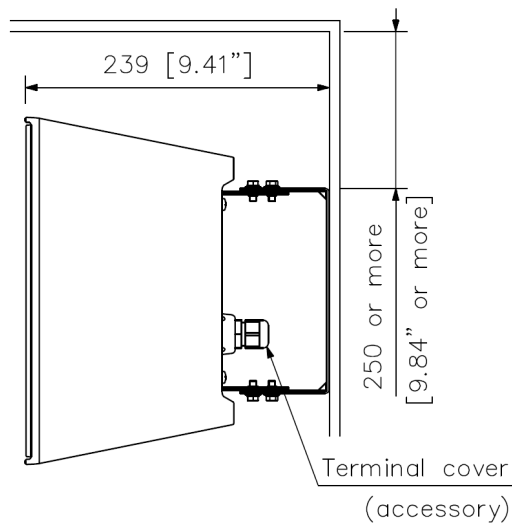
Vertical installation
