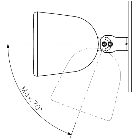
Horizontal installation
