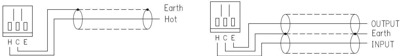
Connection Diagram
